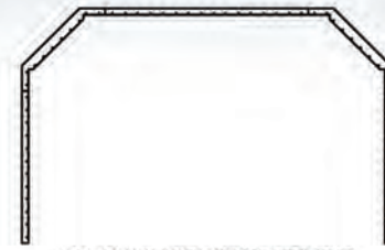
14 GA. GALV, 3" WIDTH SUPPORT STEEL STYLE
